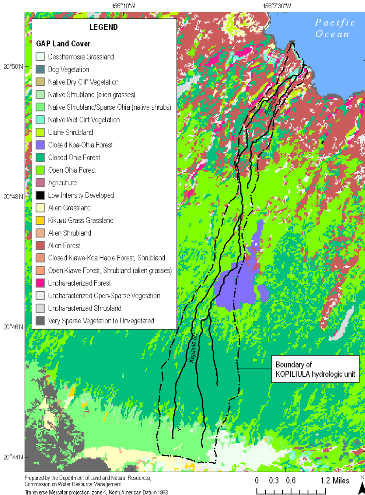
Figure 2-7. Hawaii GAP land cover classes in Kopiliula hydrologic unit (Source: Hawaii GAP Analysis Program, 2005; USGS, 2001b).
