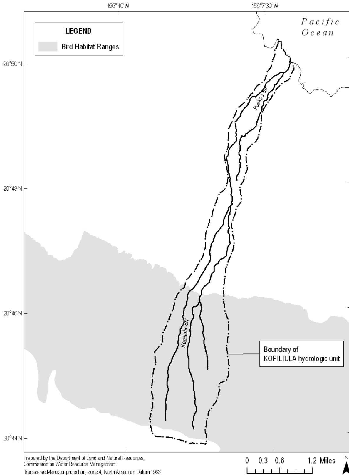
Figure 4-5. Native Hawaiian forest habitat ranges in Kopiliula hydrologic unit (Source: U.S. Fish and Wildlife Service, n.d; USGS, 2001b).
