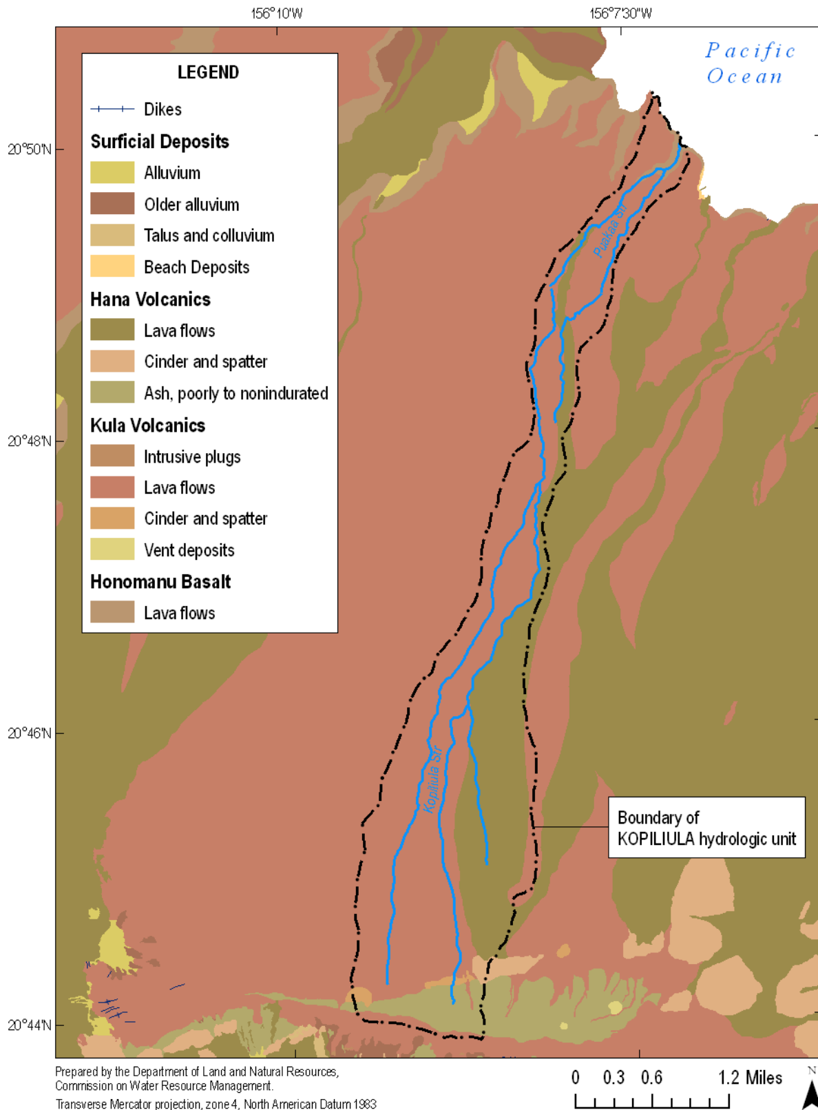
Figure 2-2. Generalized geology of Kopiliula hydrologic unit (Source: Sherrod et al., 2007; State of Hawaii, Office of Planning, 2006a, and State of Hawaii, Commission on Water Resource Management, 2008d; USGS, 2001b).
