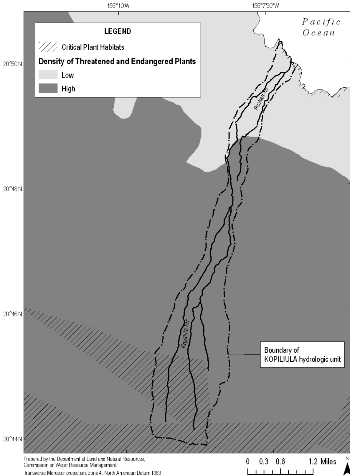
Figure 6-4. Critical plant habitats, and density of threatened and endangered plant species for Kopiliula hydrologic unit (Source: Jacobi, 1989; Scott et al., 1986; State of Hawaii, Office of Planning, 1992, 2004b; 2004d; USGS, 2001b).
