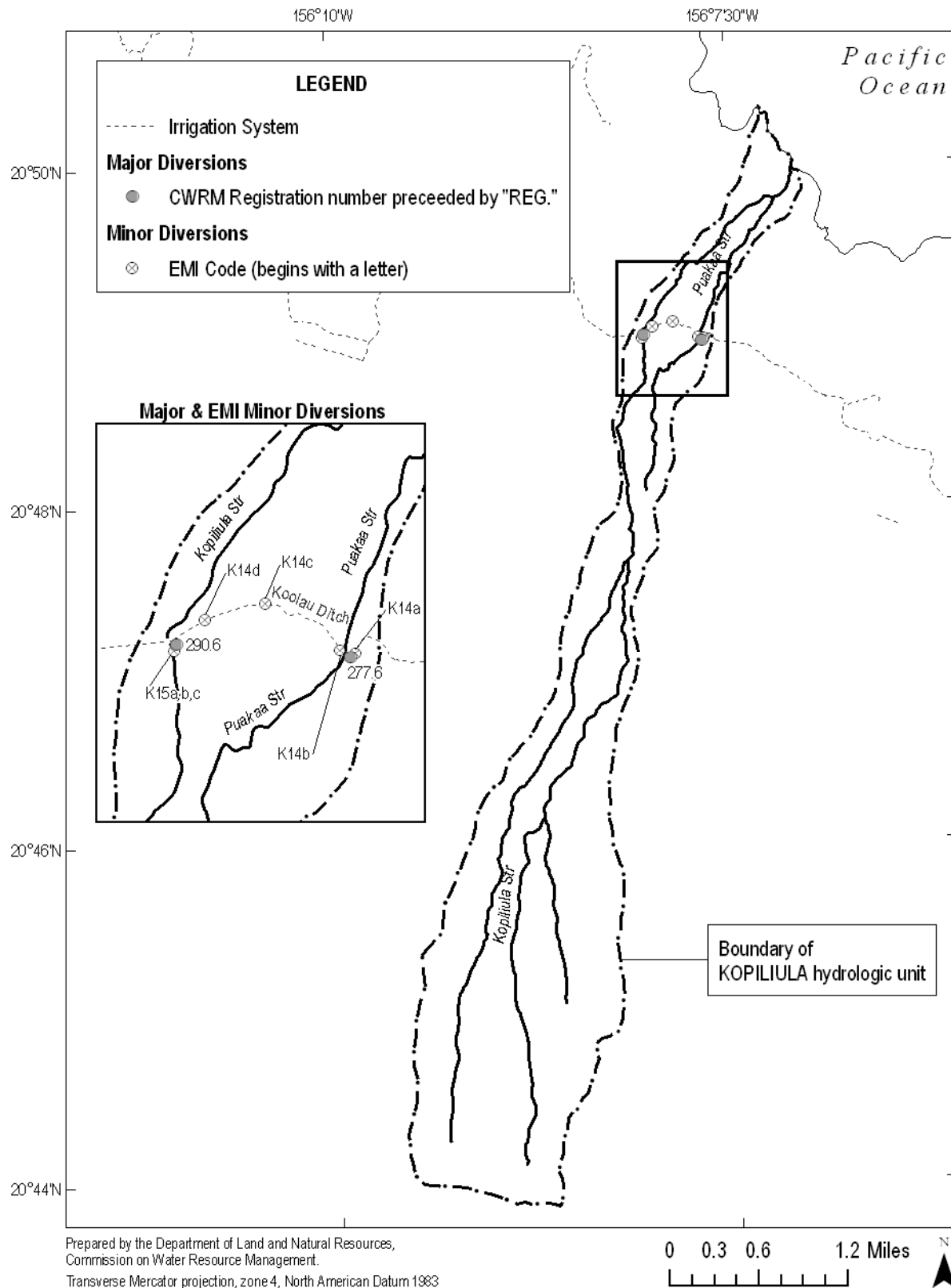
Figure 13-19. All registered diversions and EMI minor diversions identified in the Kopiliula hydrologic unit (Source: East Maui Irrigation Company, 1970; State of Hawaii, Commission on Water Resource Management, 2008f; USGS, 2001b).
