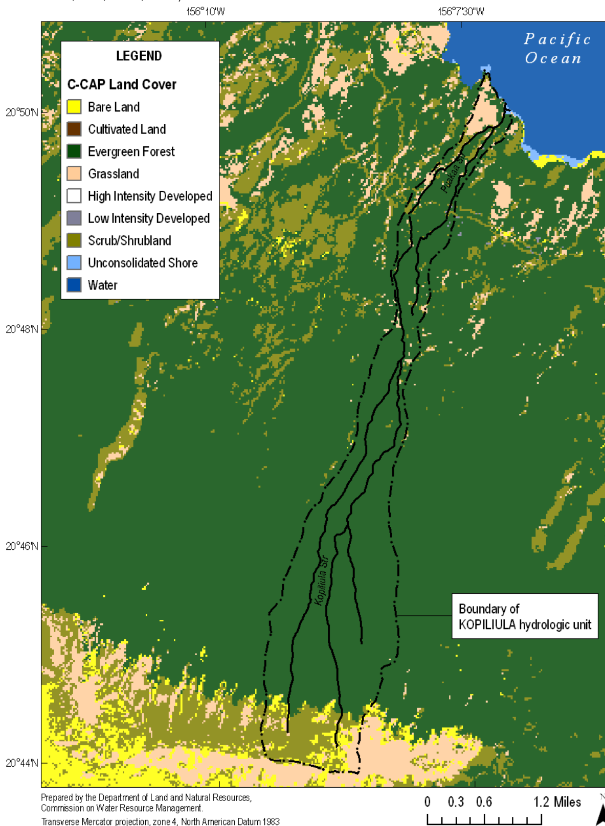
Figure 2-6. C-CAP land cover in Kopiliula hydrologic unit (Source: National Oceanic and Atmospheric Administration, Coastal Services Center, 2000; USGS, 2001b).
