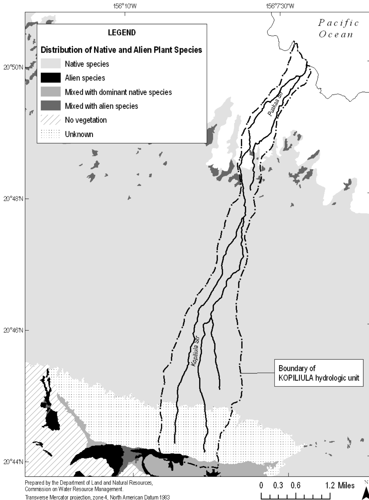
Figure 6-3. Distribution of native and alien plant species for Kopiliula hydrologic unit (Source: Jacobi, 1989; Scott et al., 1986; State of Hawaii, Office of Planning, 1992, 2004b; 2004d; USGS, 2001b).
