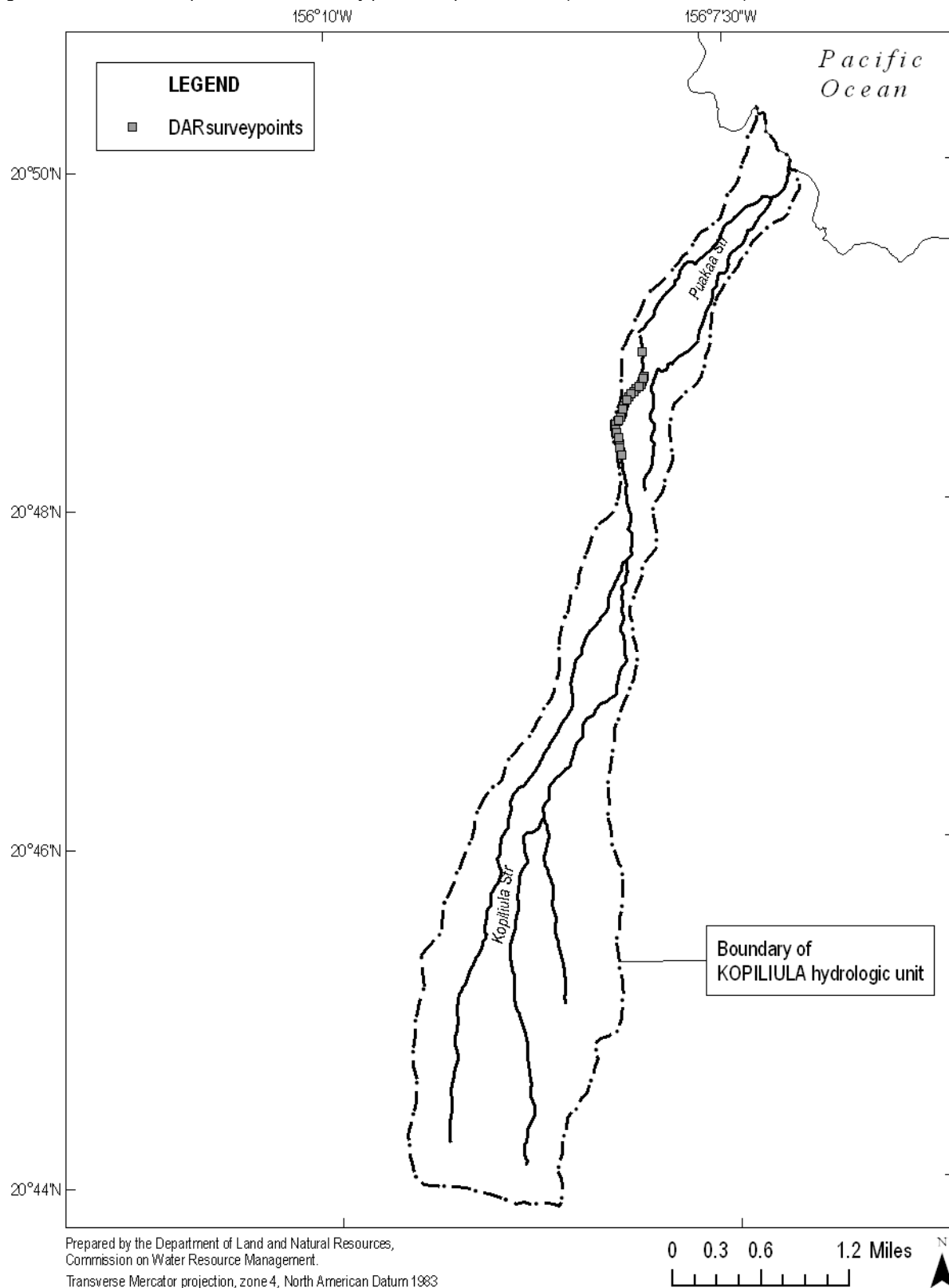
Figure 4-4. Division of Aquatic Resource survey point in Kopiliula Stream (Source: USGS, 2001b).
