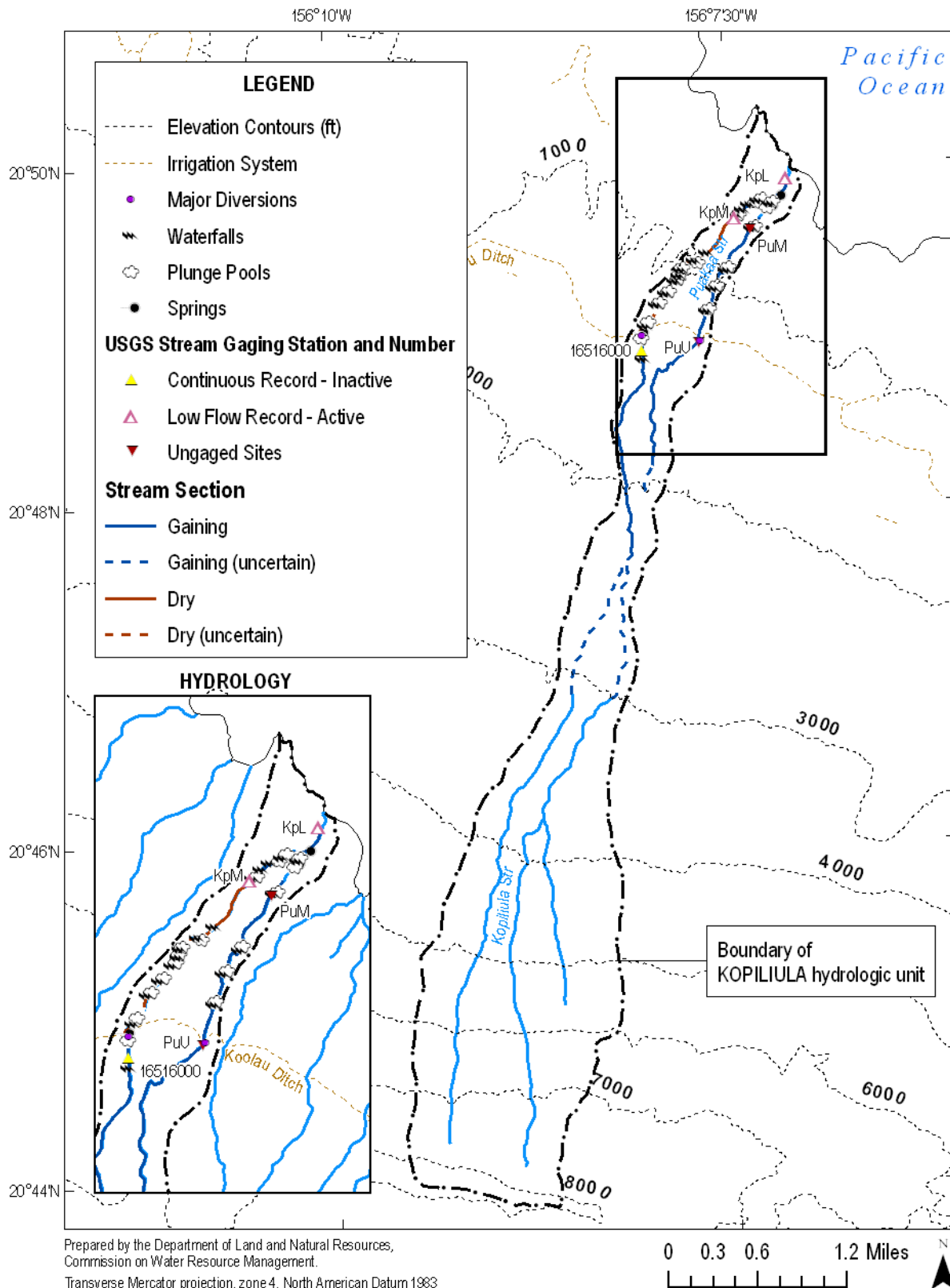
Figure 3-3. Location of diversions, irrigation systems, USGS gaging stations, and selected ungaged sites in Kopiliula hydrologic unit (Source: State of Hawaii, Office of Planning, n.d.; 1996, 2004c; 2005; USGS, 2001b).
