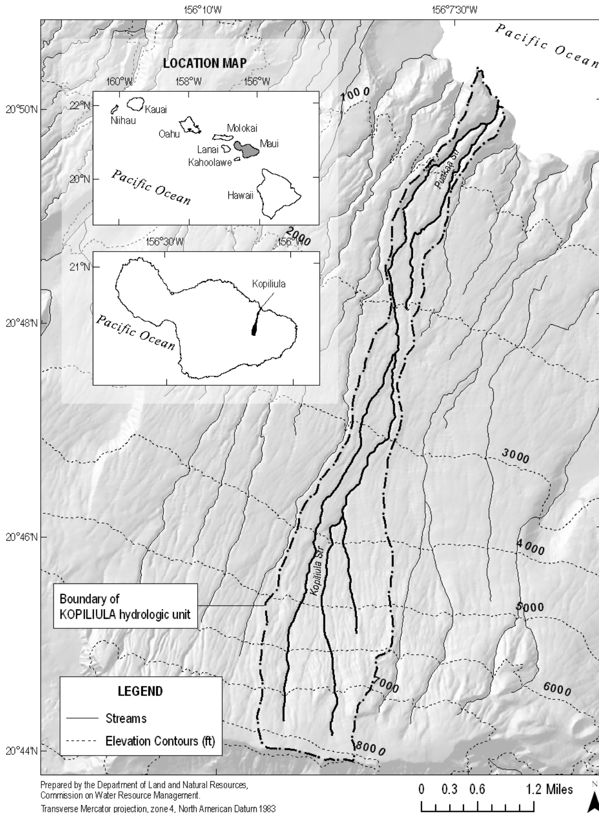
Figure 1-4. Elevation range and the location of Kopiliula hydrologic unit. (Source: State of Hawaii, Office of Planning, 1983; USGS, 2001b).
