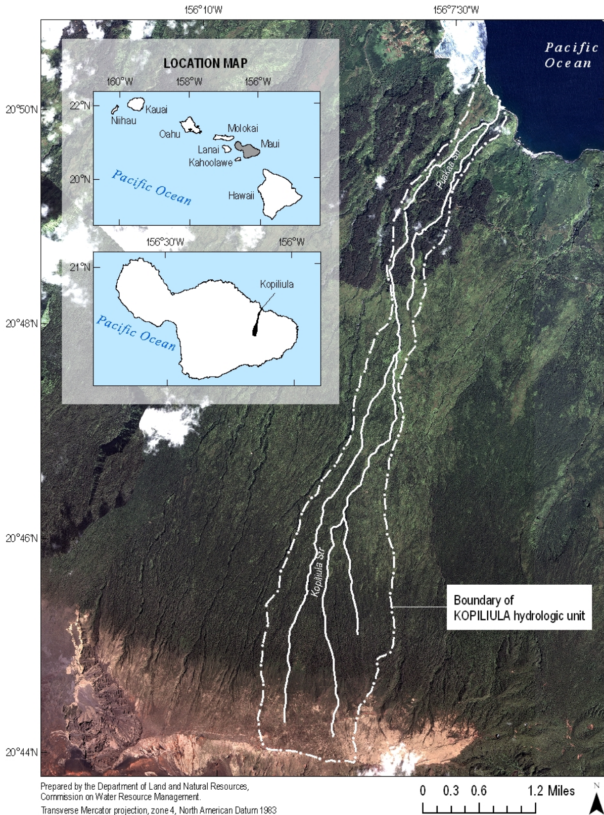
Figure 1-6. Quickbird satellite imagery of Kopiliula hydrologic unit (Source: County of Maui, Planning Department, 2004; USGS, 2001b).
