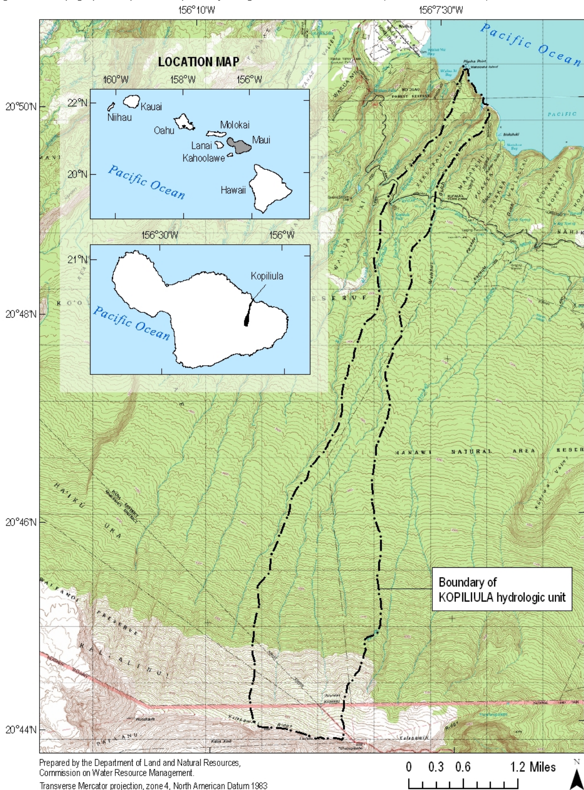
Figure 1-3. Topographic map of the Kopiliula hydrologic unit in east Maui, Hawaii (Source: USGS, 1996).
