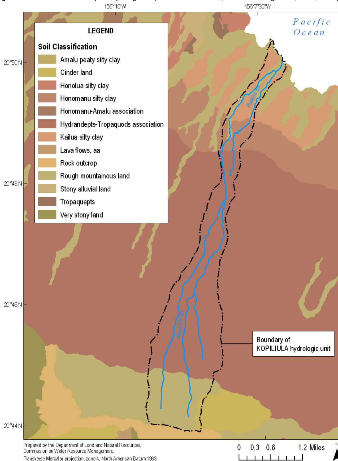
Figure 2-3. Soil classification in Kopiliula hydrologic unit (Source: State of Hawaii, Office of Planning, 2007c; USGS, 2001b).
