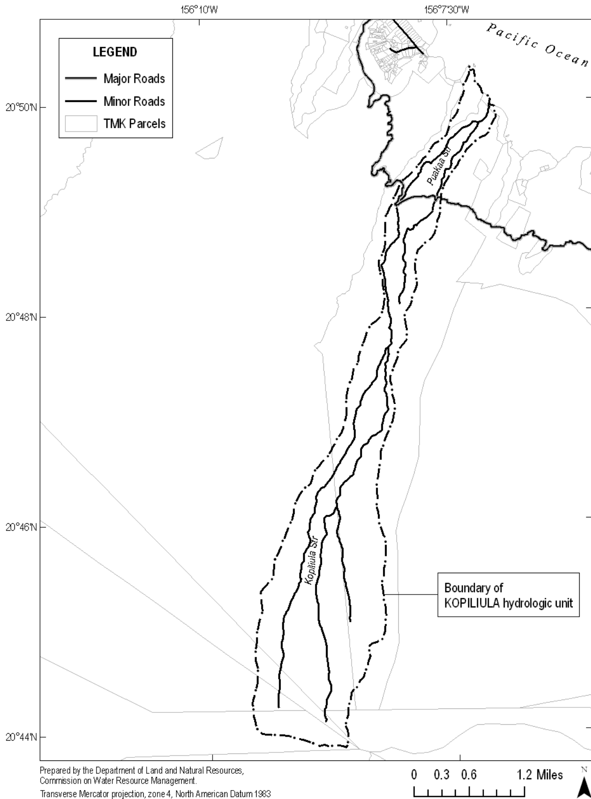
Figure 1-5. Major and minor roads and Tax Map Key (TMK) parcel boundaries for Kopiliula hydrologic unit (Source: County of Maui, 2006; County of Maui, Geographic Information Systems [GIS] Division, Department of Management, 2006; USGS, 2001b).
