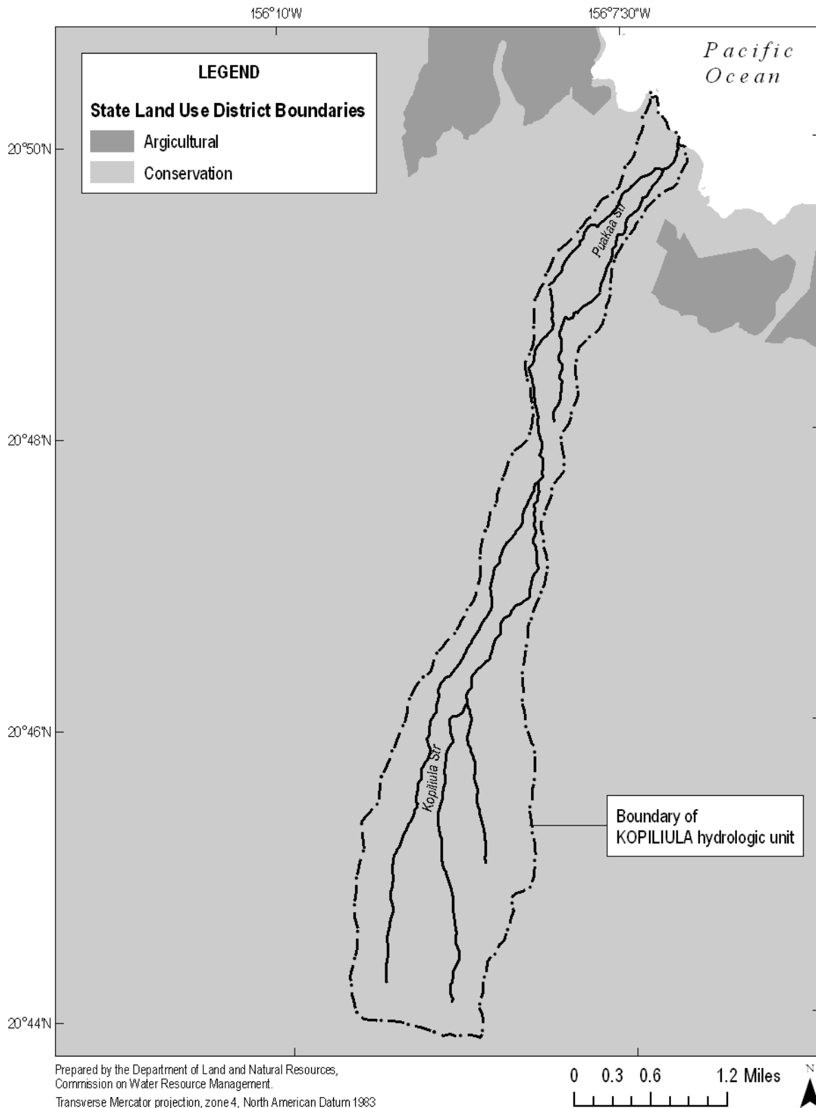
Figure 2-5. State land use district boundaries in Kopiliula hydrologic unit (Source: State of Hawaii, Office of Planning, 2006d; USGS, 2001b).
