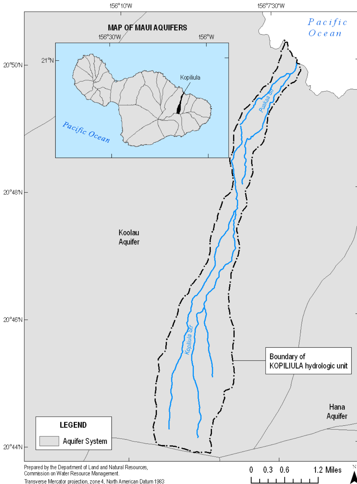
Figure 3-2. Aquifer system area and well locations in Kopiliula hydrologic unit (Source: State of Hawaii, Office of Planning, 2006b; State of Hawaii, Commission on Water Resource Management, 2008d; USGS, 2001b).
