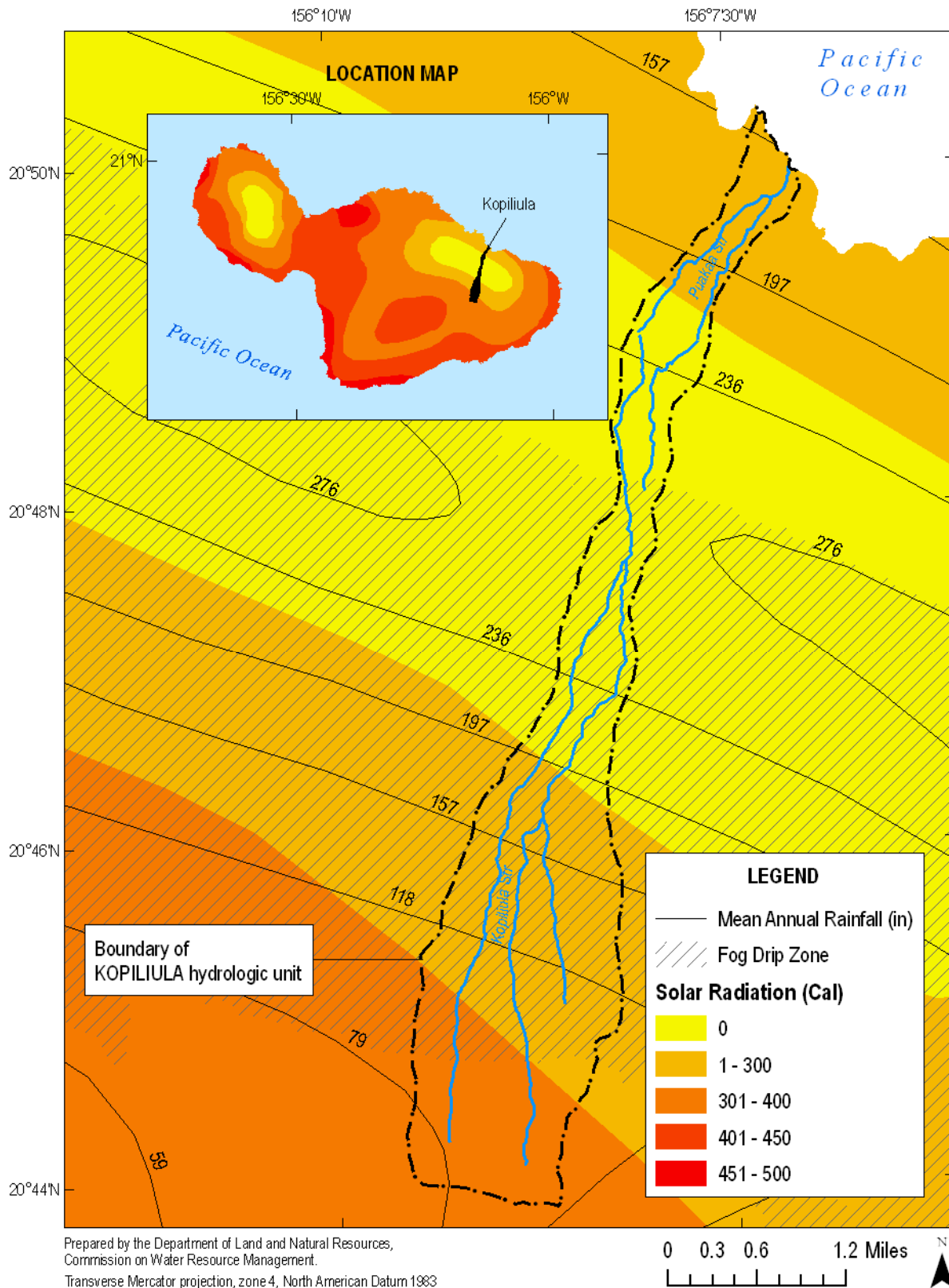
Figure 2-4. Mean annual rainfall and fog area in Kopiliula; and solar radiation for Kopiliula and the island of Maui, Hawaii (Source: Giambelluca et al., 1986; State of Hawaii, Office of Planning, 2006b; 2006c; USGS, 2001b).
