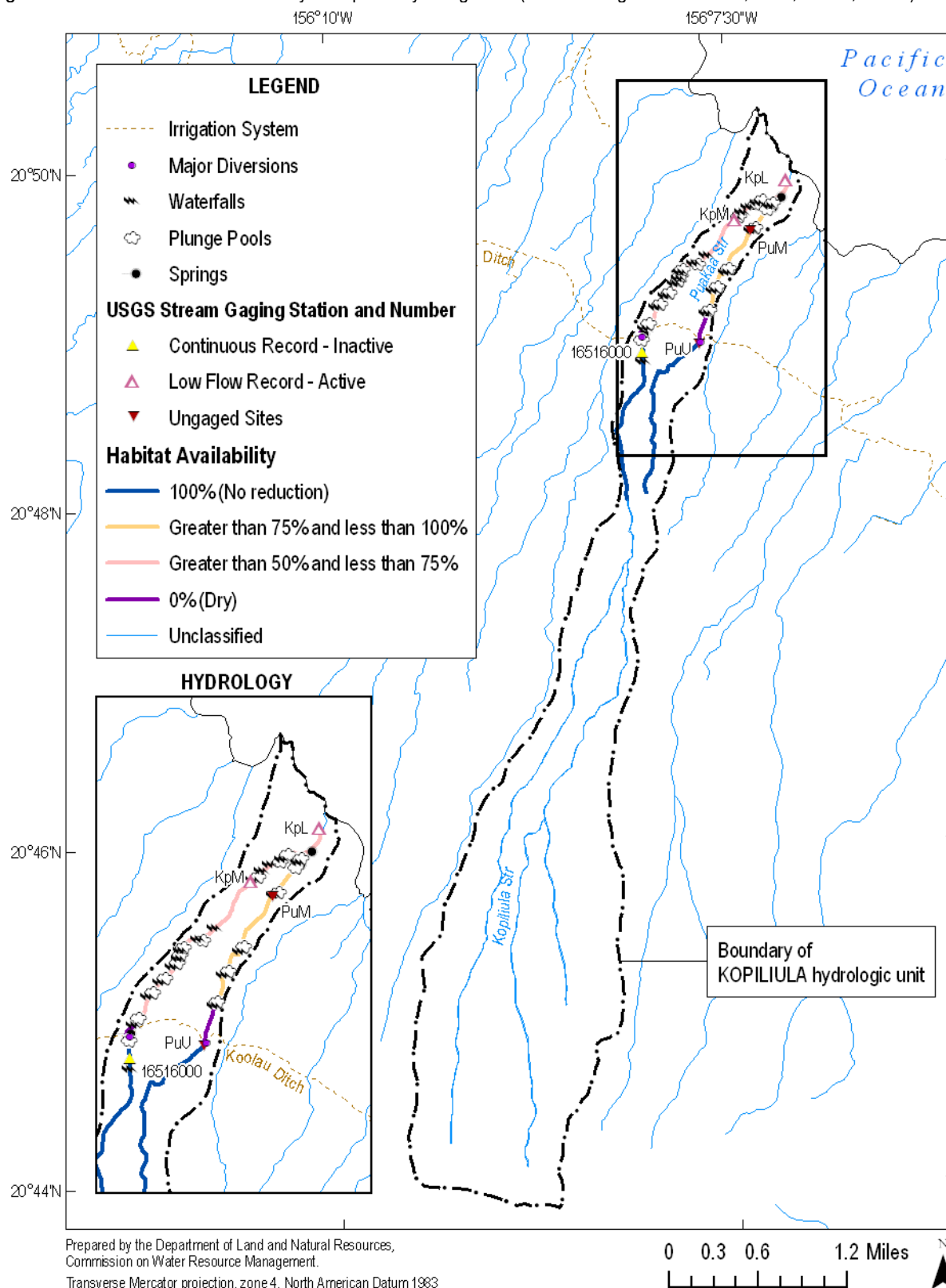
Figure 4-3. Estimated habitat availability in Kopiliula hydrologic unit (Source: Gingerich and Wolff, 2005; USGS, 2001b).
