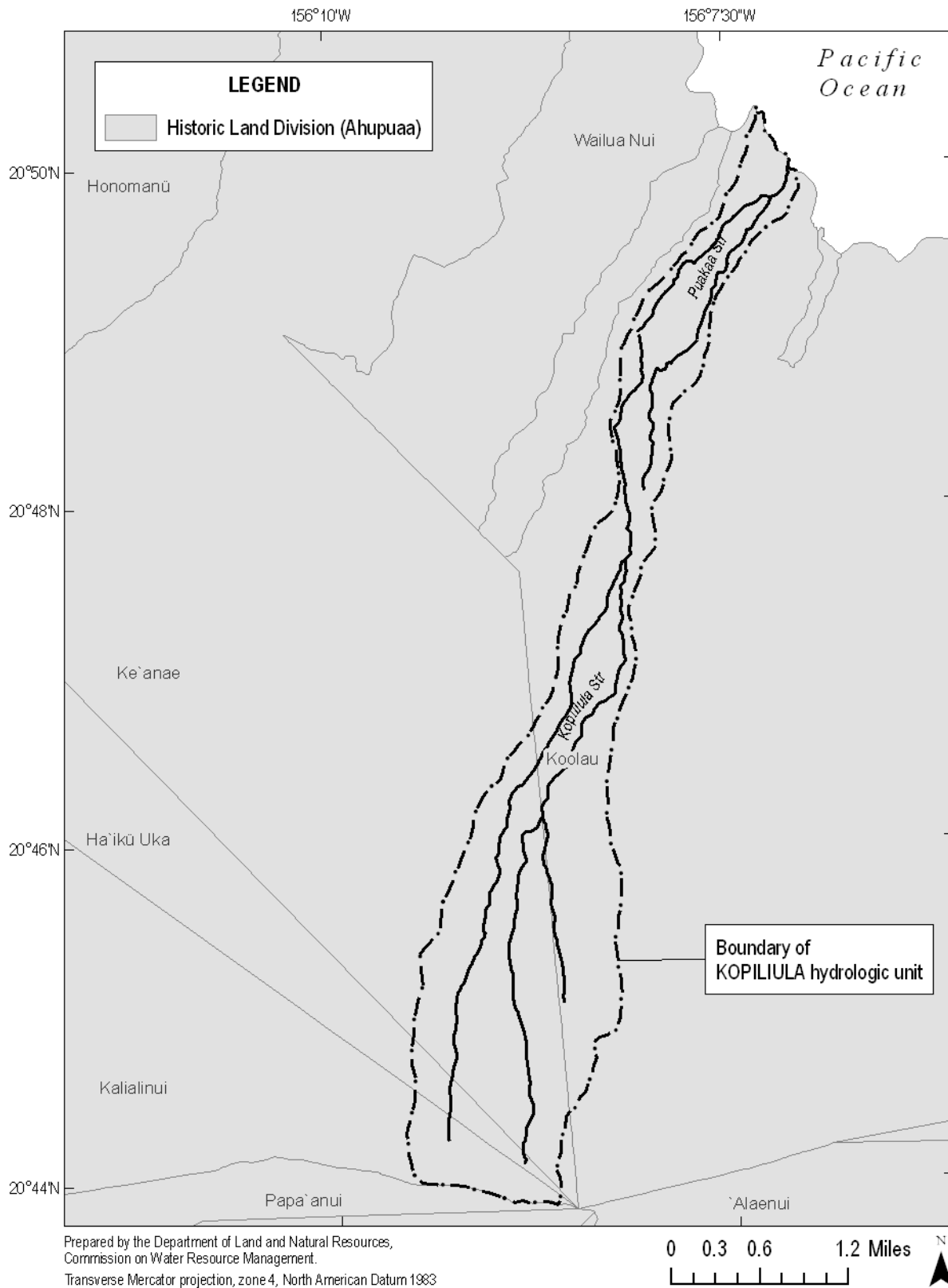
Figure 12-2. Traditional ahupuaa boundaries in the vicinity of Kopiliula hydrologic unit. This hydrologic unit spans four ahupuaa — Koolau, Keanae, Haiku Uka, and Kalialinui (Source: State of Hawaii, Office of Planning, 2007a; USGS, 2001b).
